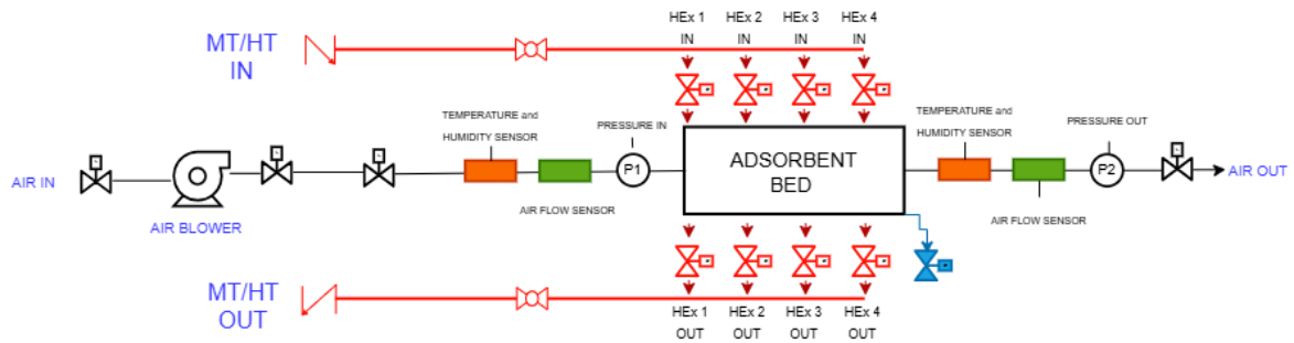
Fig. 1: Simplified schematic of a single adsorption bed of the prototype showing the air flow circuit and the water thermal circuit.
