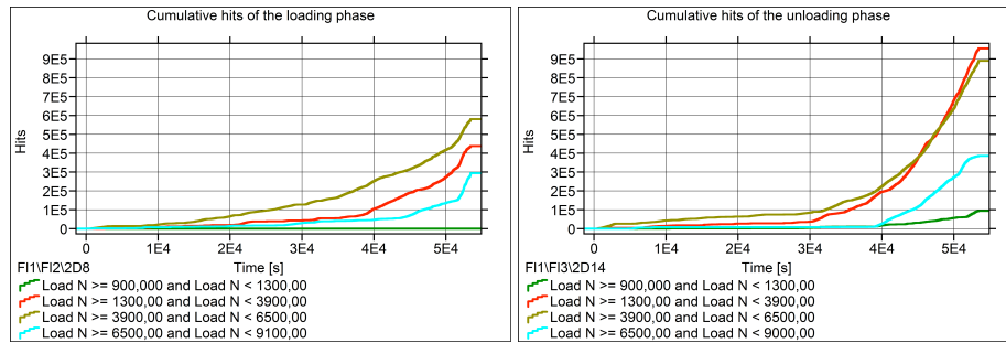
Figure 6. Cumulative number of hits per four loading ranges for the loading (left) and unloading (right) for a specimen loaded at 55%
