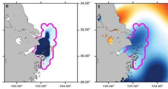
Modelled annual sedimentation at the mouth of the Yangtze river ; right : equivalent sedimentation observed by GRACE (Mouyen et al., 2018). Dark blue : 3mm/yr.
