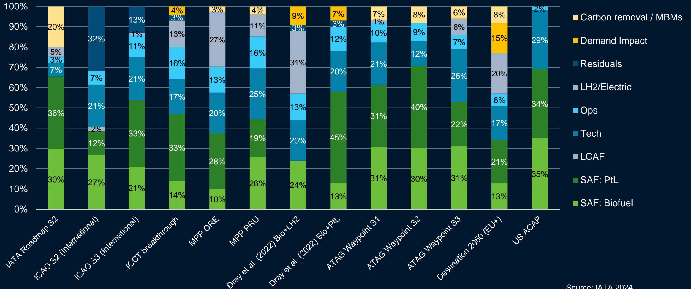
Emissions Reduction Potential by Transition Measures In 2050
