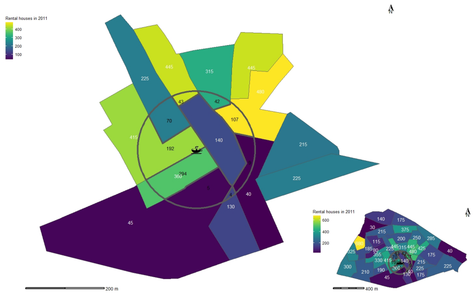
Figure AV: Instrumental variable construction
