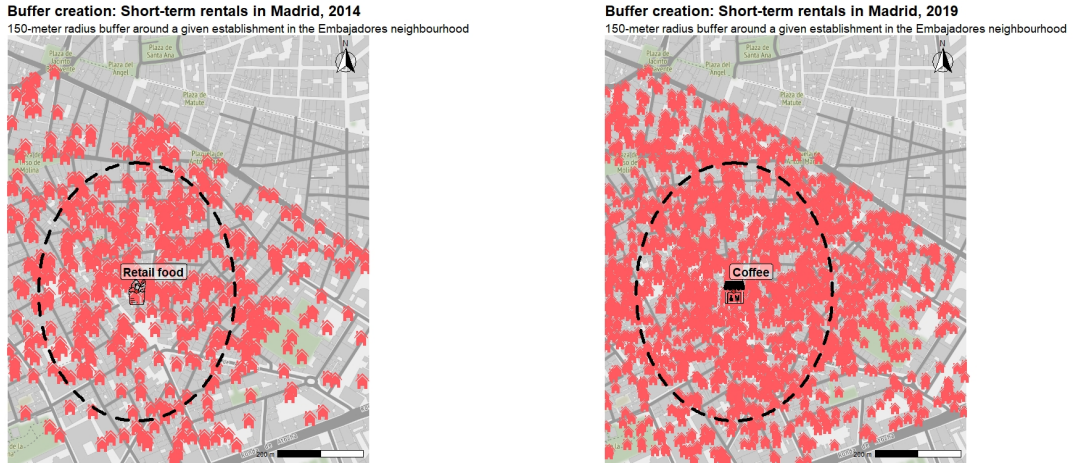
Figure II: Buffer creation
