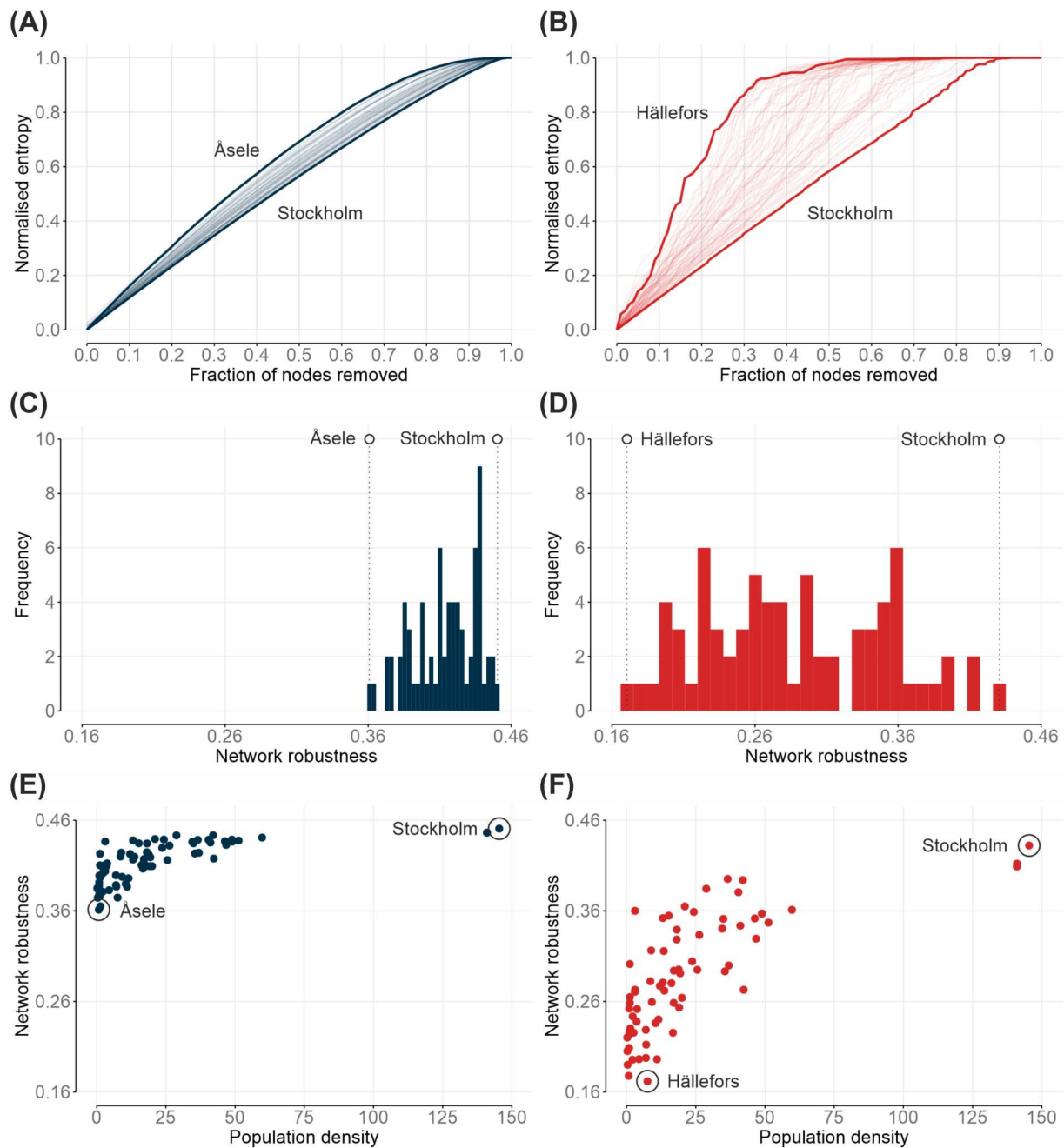
Figure 2. Descriptive information about the robustness of local labour flow networks: (A, B) normalised entropy as the fraction of nodes removed increases; (C, D) distribution of network robustness measures against random and targeted elimination strategies, respectively; and (E, F) population density and network robustness against random or targeted elimination. Note: Blue represents the results on random elimination, red on targeted elimination.
