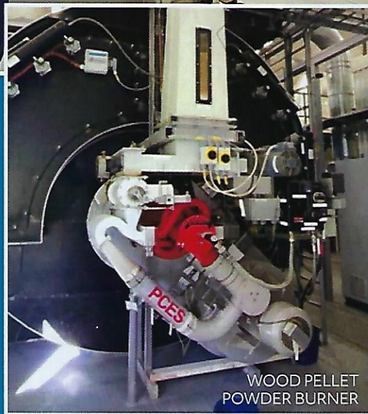
BIO POWDER BURNER 16MW
