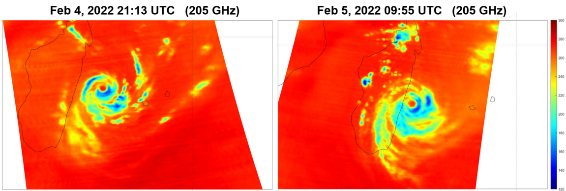
Fig. 4. Cyclone Batsirai as observed by the TROPICS Pathfinder at 205 GHz on February 4 and 5, 2022. The colorbar indicates the brightness temperature in units of Kelvins.
