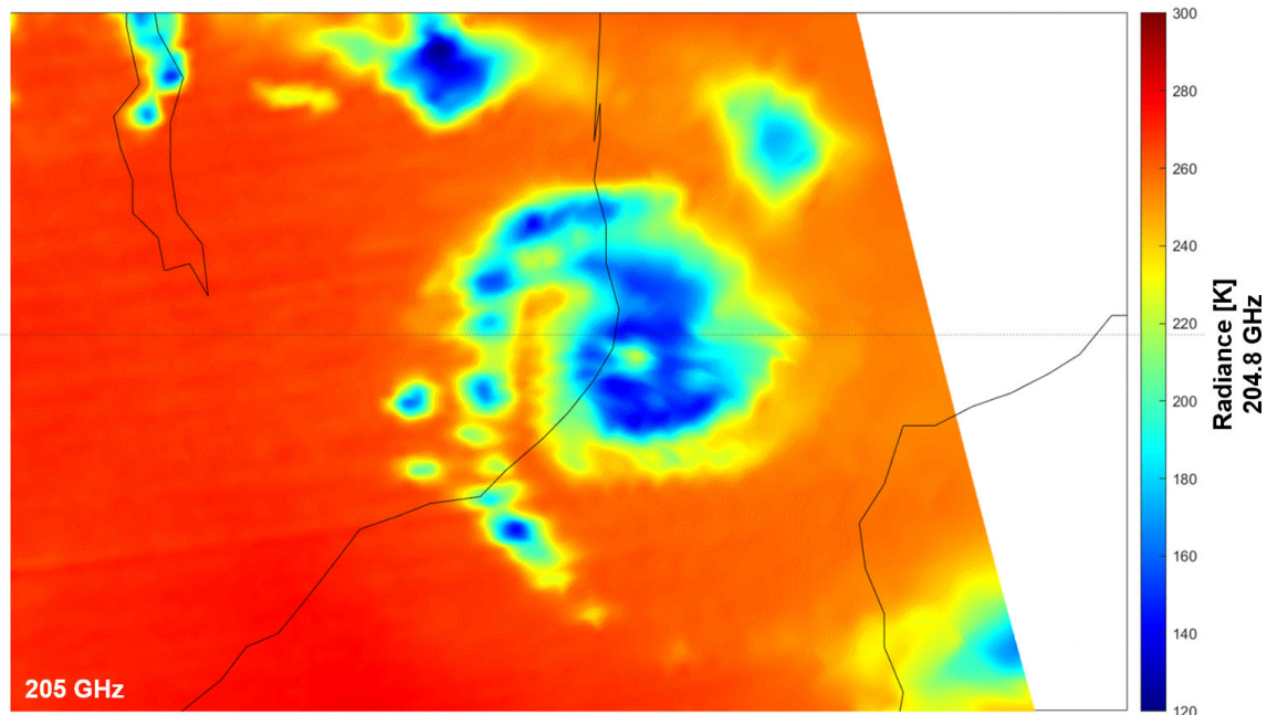
Fig. 5. Cyclone Gombe as observed by the TROPICS Pathfinder at 205 GHz on March 10, 2022 (22:24 UTC).
