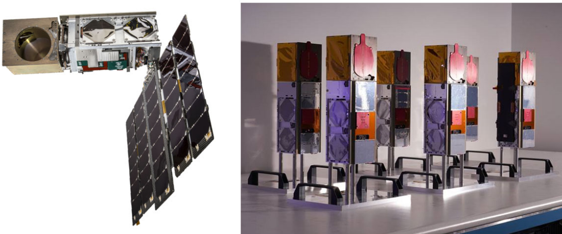
Fig. 1. TROPICS satellite (left), showing the rotating payload connected to the satellite bus via a rotary joint. Also shown in the image on the left is the articulating solar array, which rotates (as does the satellite bus) to track the sun to maximize power output. The six satellites that will comprise the constellation are shown on the right.
