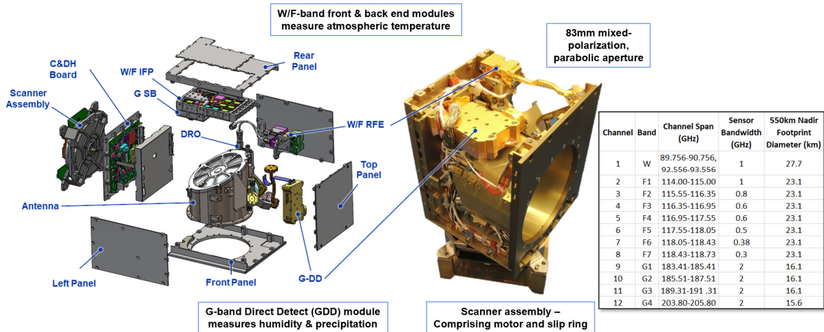
Fig. 2. Overview and characteristics of the TROPICS radiometer payload.
