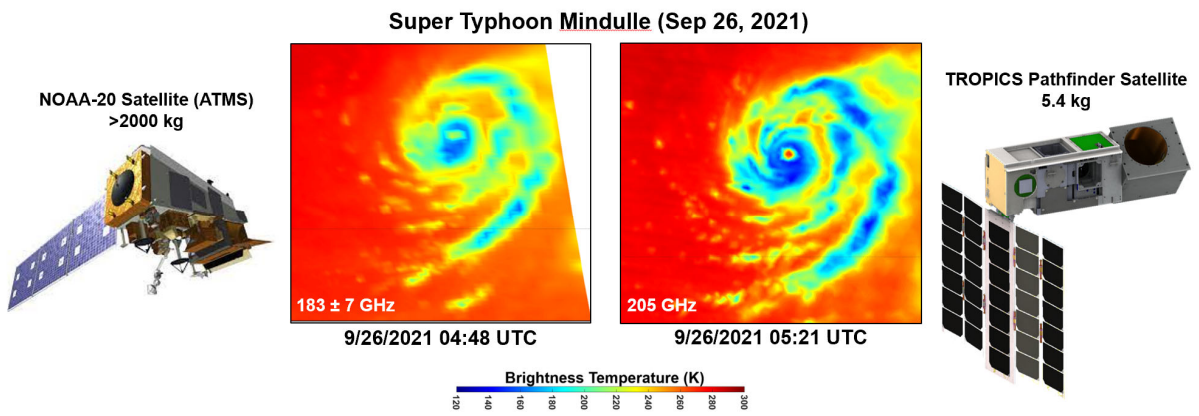
Fig. 3. Super Typhoon Mindulle as observed by the Advanced Technology Microwave Sounder (ATMS) on the NOAA-20 satellite and by the TROPICS Pathfinder satellite.
