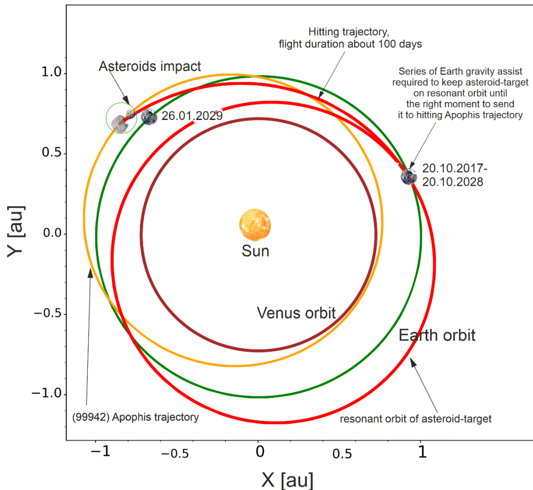
Fig. 10. Trajectory of the projectile asteroid before the collision with Apophis in the heliocentric (J2000) ecliptic coordinate system.
