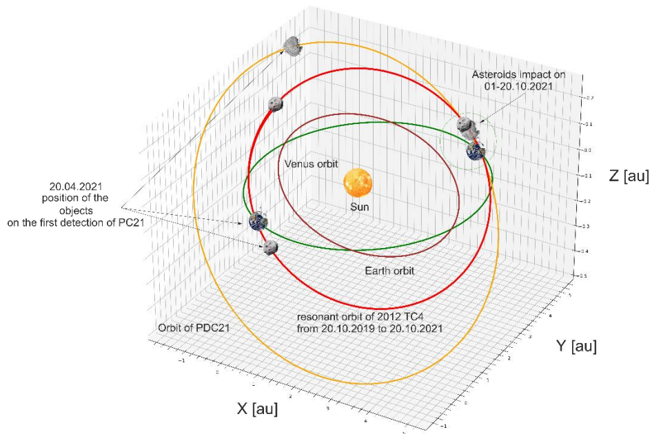
Fig. 8. Trajectory of the projectile asteroid before approaching PDC21 in the heliocentric (J2000) ecliptic coordinate system.
