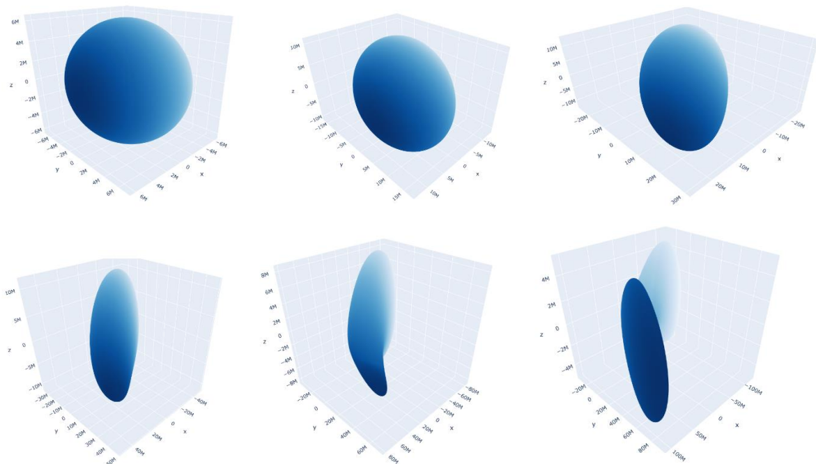
Fig. 4. Deformation of sphere through 1 to 6 month from Earth gravity assist in Sun-Earth rotating frame
