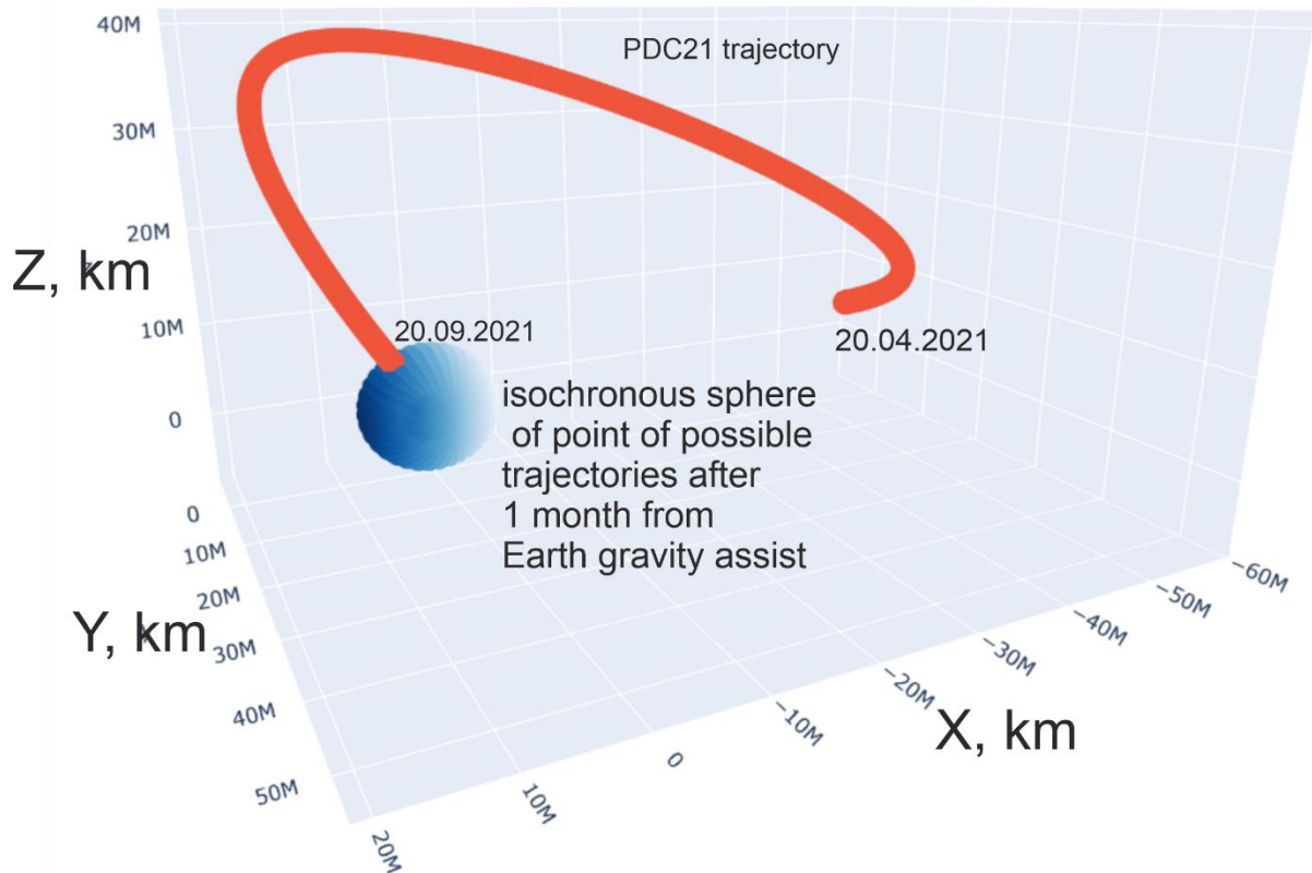
Fig. 11. Trajectory of the virtual asteroid PDC21 from 20.04.2021 to the moment of crossing the sphere on 20.09.2021.
