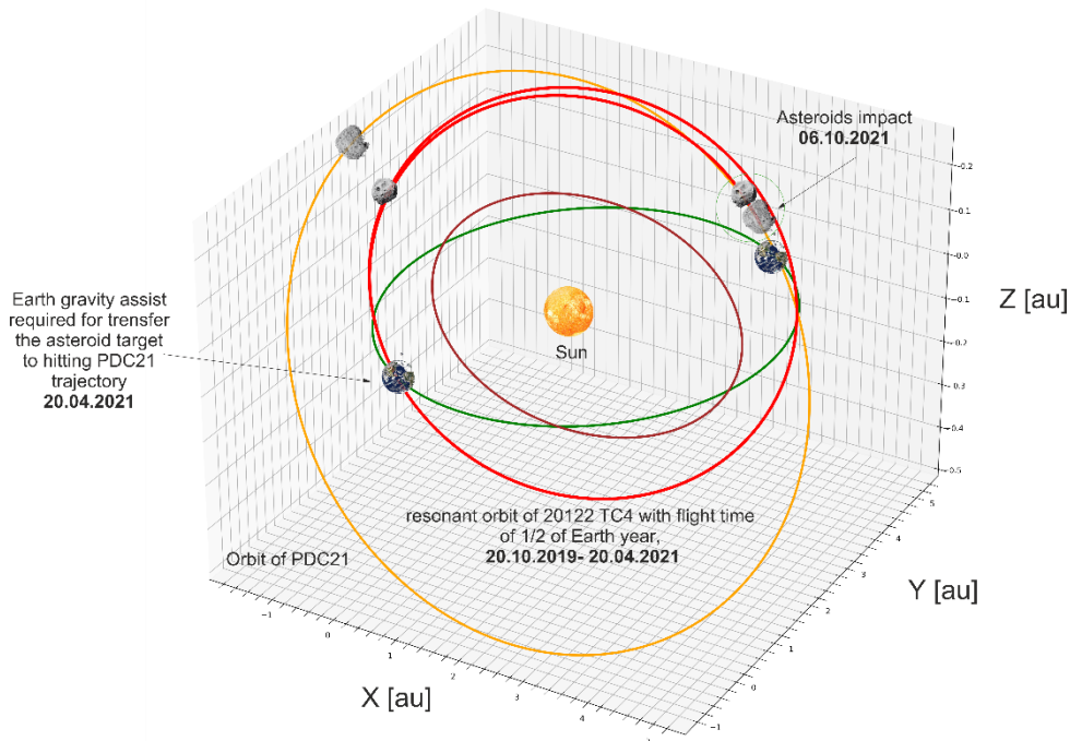
Fig. 9. Trajectory of the projectile asteroid before the collision with PDC21 in the heliocentric (J2000) ecliptic coordinate system.
