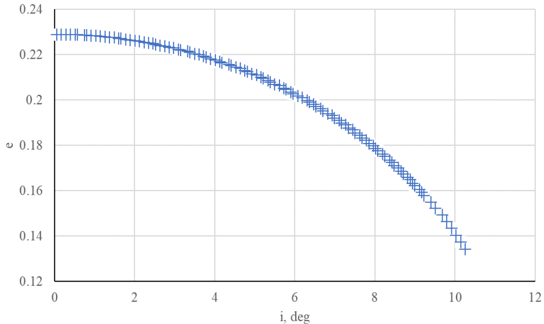
Fig. 6. Eccentricity of the resonant orbit versus the inclination
