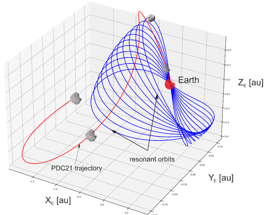
Fig. 7. Trajectory of potentially dangerous object (PDC21) before its possible collision with the Earth on October 20, 2021 in the geocentric (J2000) ecliptic coordinate system.
