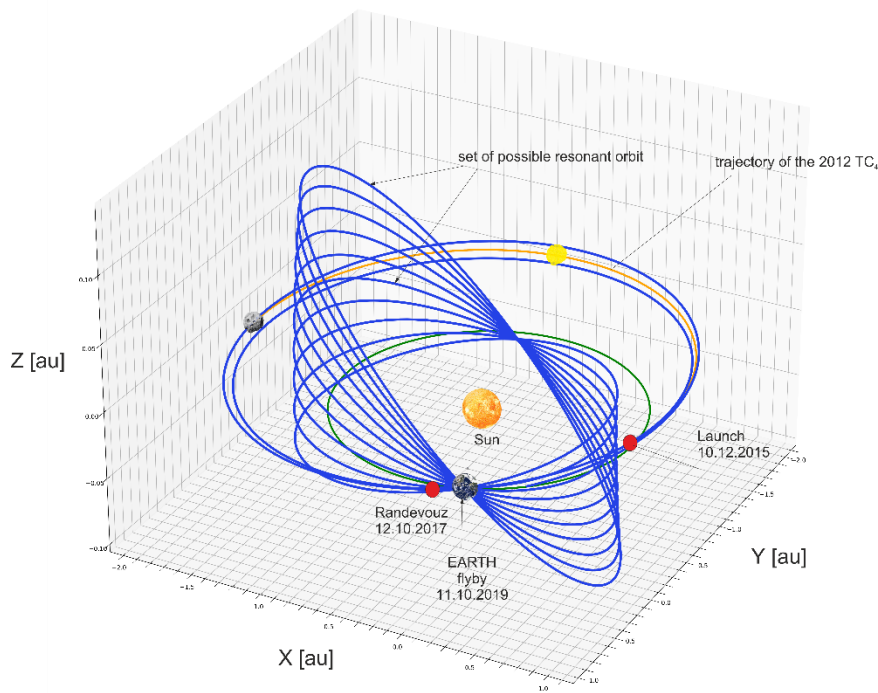
Fig. 5. Trajectory of the flight to the asteroid 2012 TC4 with its subsequent transfer to the resonant 1:1 orbit to the Earth.
