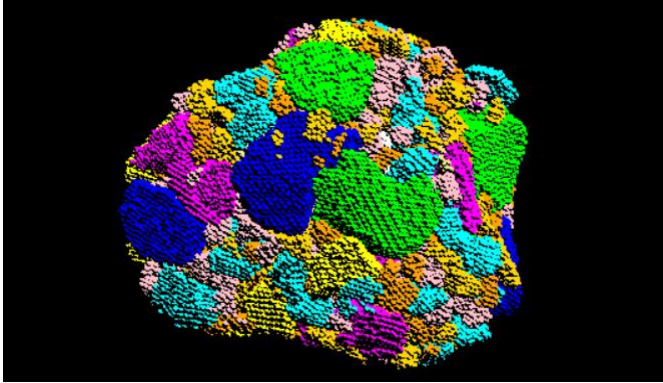
Fig. 3. Resulting Apophis model from SHEXSSPY method.
