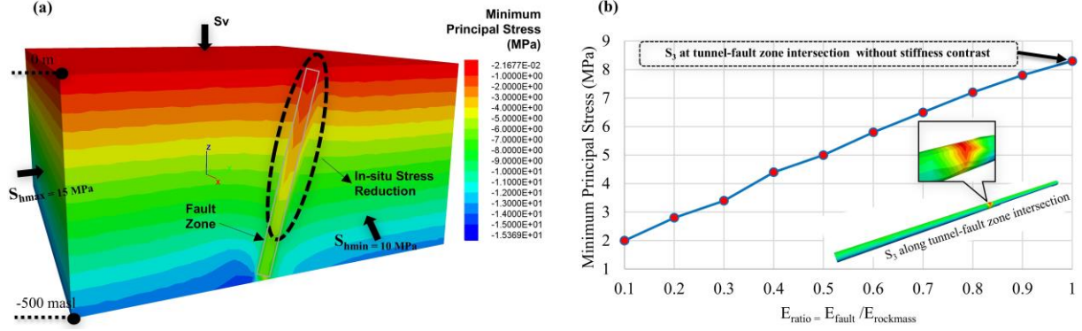
Figure 3: (a) Reduction of minimum principal stress (MPa) in the 3D block under maximum stiffness contrast between rock mass and fault zone. (b) S_3 variation along tunnel-fault zone intersection area with various stiffness ratio
