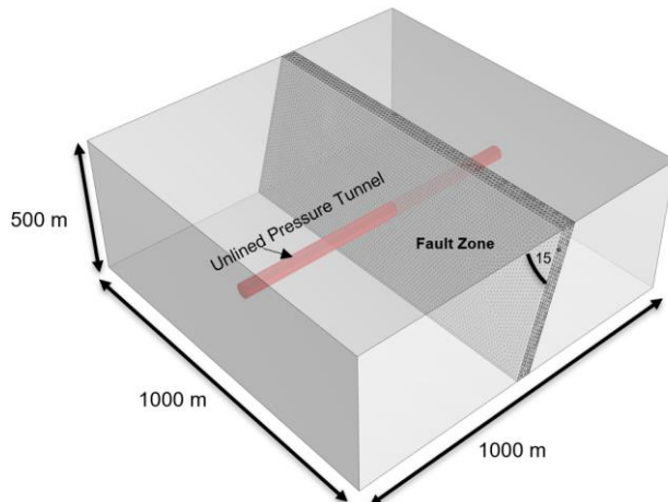
Figure 1: A generic 3D model with model extent
