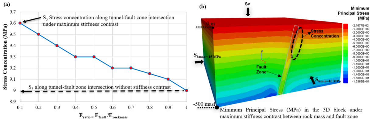
Figure 5: (a) Minimum Principal Stress concentration along the tunnel-fault zone under various stiffness contrast, (b) 3D block representing minimum principal stress under maximum stiffness contrast.
