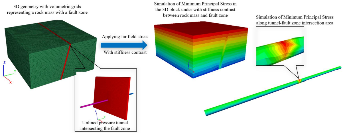
Figure 2: 3D model illustrating rock mass block, fault zone volume grids (left) and 3D numerical model for minimum principal stress assessment (right)
