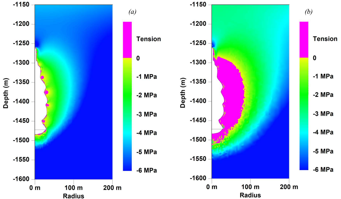
Fig. 6 Effective stress at the end of debrining (a) and at the end of cyclic loading (b).
