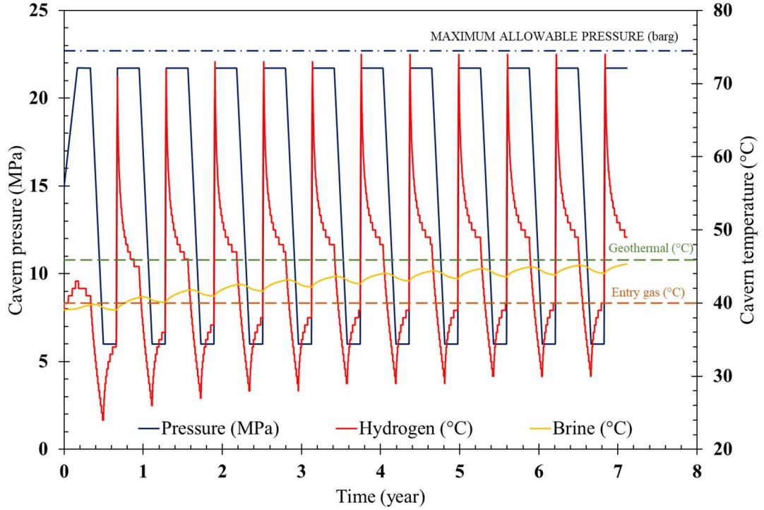
Fig. 1 Evolution of cavern pressure and temperature at cavern mid-depth (1,373 m).
