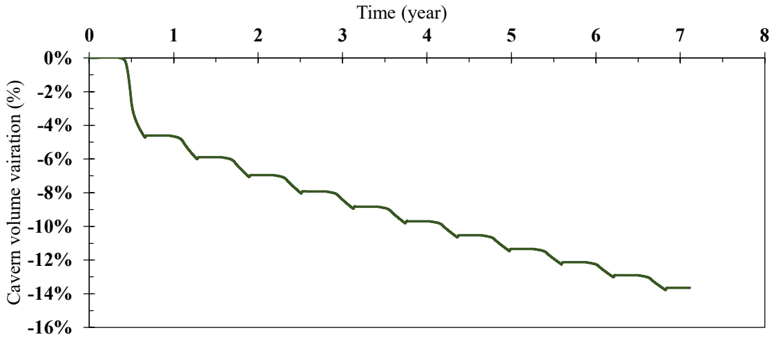
Fig. 4. Cavern volume variation during cyclic loading.
