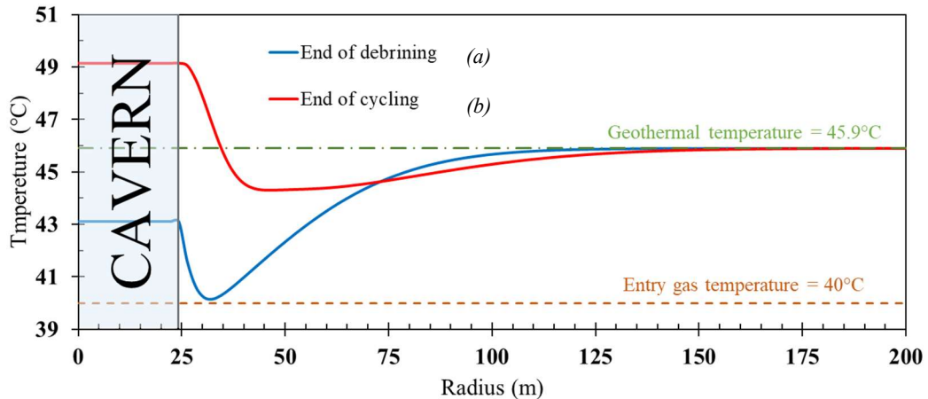
Fig. 2 Radial distribution of temperature at cavern mid-depth (1,373 m) at the end of debrining (a) and at the end of cyclic loading (b).
