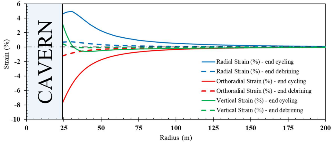
Fig. 7 Strains distribution ( \varepsilon_{rr} , \varepsilon_{tt} and \varepsilon_{zz} ) at cavern mid-depth (1,373 m).
