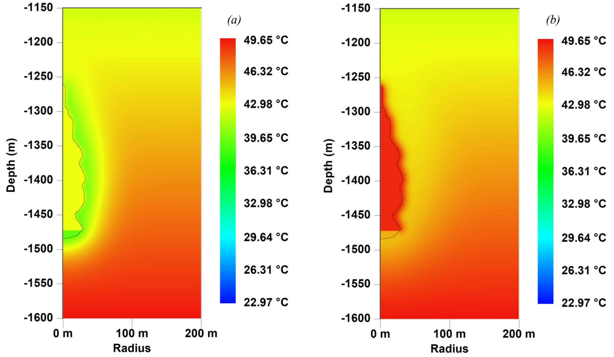
Fig. 3 Contours plot of the temperature at the end of debrining (a) and at the end of cyclic loading (b).
