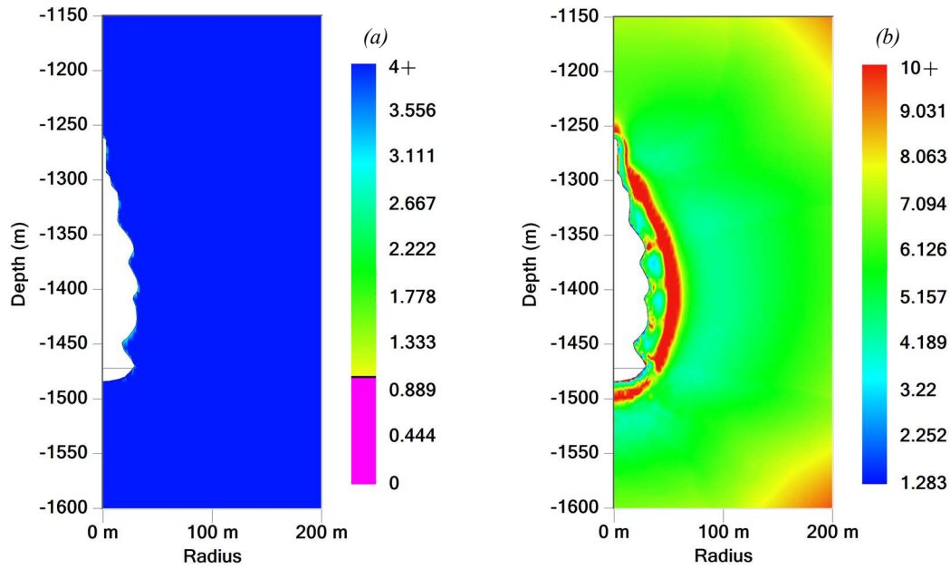
Fig. 9. Factor of safety ( FoS ) at the end of cyclic loading for Spiers (a) and DeVries (b) criteria.
