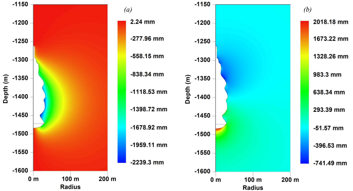
Fig. 8. Radial (a) and vertical (b) displacement at the end of cyclic loading.
