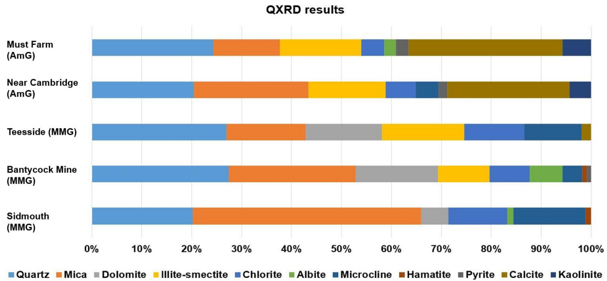
Fig. 3: A summary of QXRD results (averaged for each location).
