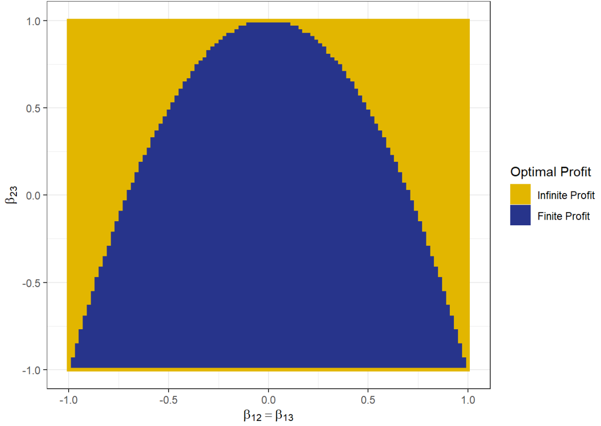
Figure 2: Two-way Complementarities, when \beta_{123} = 0
