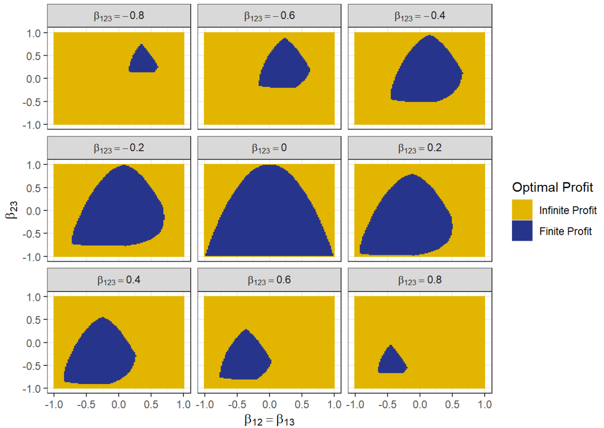
Figure 2: Two-way Complementarities, when \beta_{123} changes
