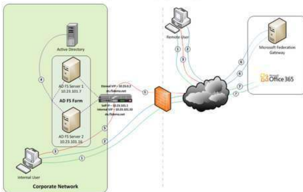
Figure 2 - BIG-IP with APM replacing the ADFS Proxy layer
