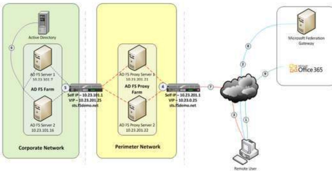
Figure 1 – BIG-IP load balancing and optimizing ADFS and ADFS Proxy
