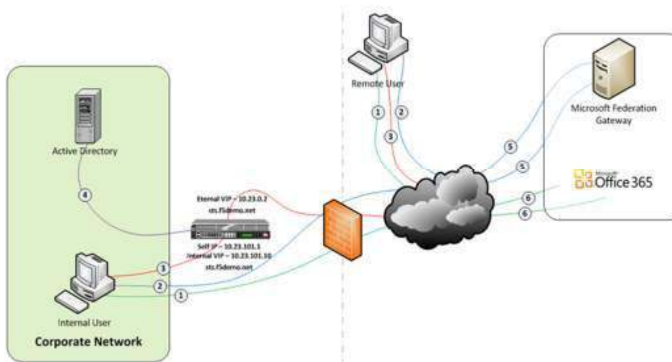
Figure 3 – BIG-IP with APM replacing the entire ADFS infrastructure
