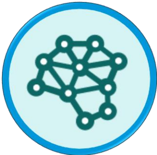
Big Data
