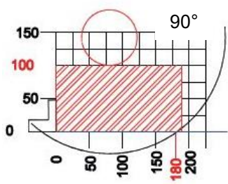
KD350 Cut Chart
