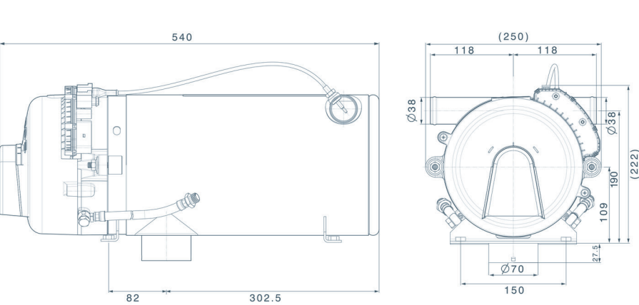
Installation dimensions for Thermo plus
