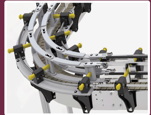
Easy Adjust Guide Rails
