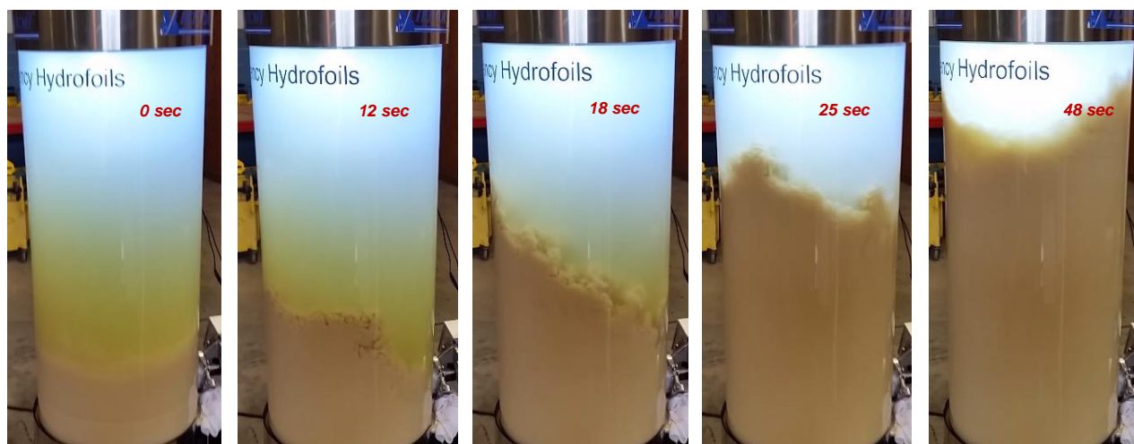
PROGRESS OF SUSPENSION OF SOLIDS (time in seconds) Demonstration tank solution 15% solids; 210lt
