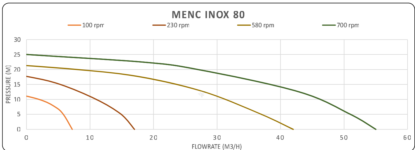
Menc Inox 80 – Marksman Package
