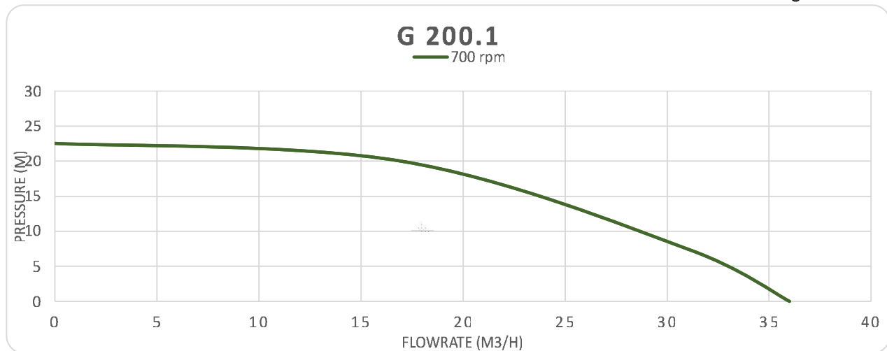
G 200.1 Marksman Package
