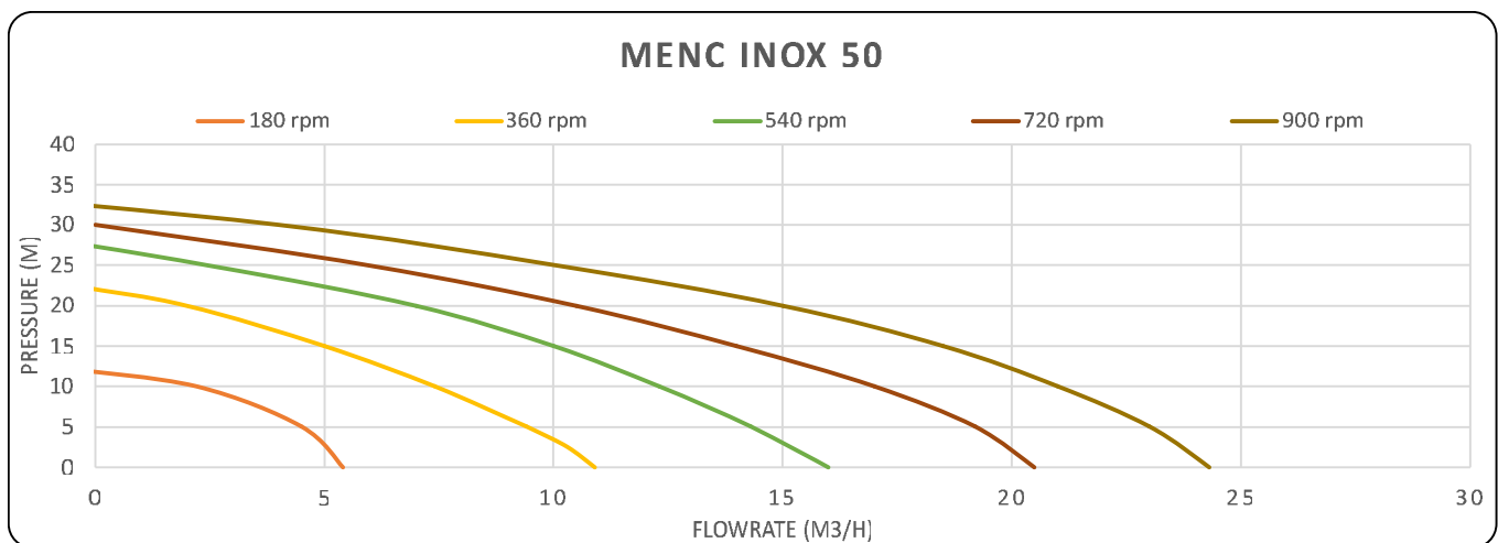
Menc Inox 50 – Elite Package
