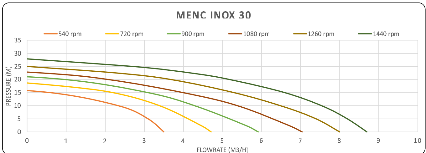
Menc Inox 30 – Professional Package
