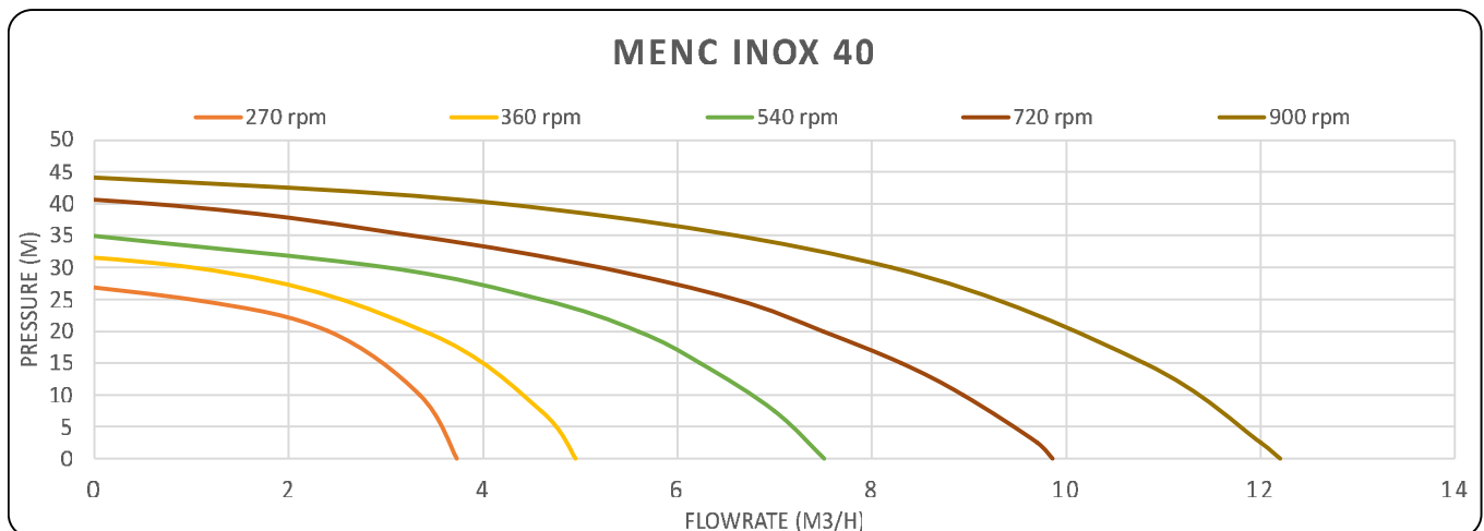
Menc Inox 40 – Professional Package
